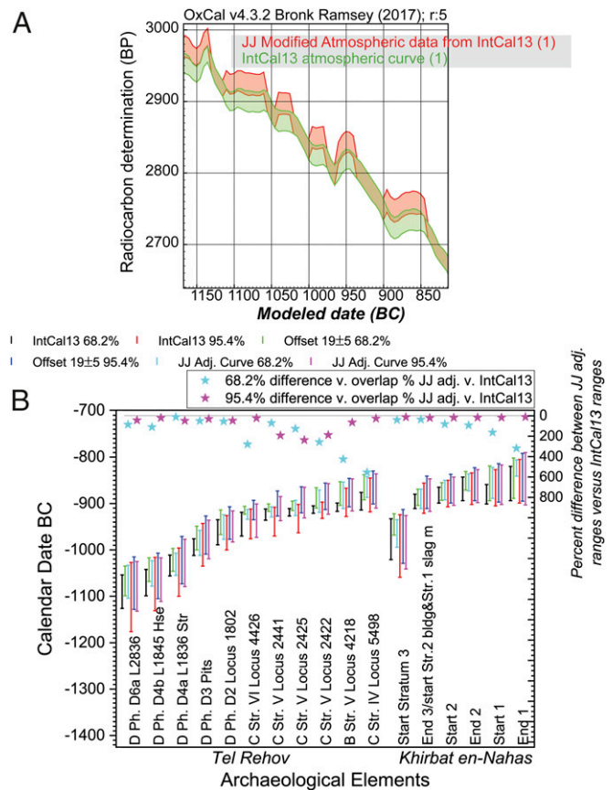
Fig. 4. (A) IntCal13 14 C calibration curve ~1200–700 BC approximately adjusted by 24 \pm 5 14 C years in the periods where curve taphonomy suggests a substantive JJ offset might apply based on Fig. 2 and SI Appendix, Fig. S3 (27). (B) (Bottom, vertical bars) Comparison of the calibrated calendar age ranges at 68.2% and 95.4% probability with, and without, both the average 19 \pm 5 14 C years offset or the approximate JJ adjusted IntCal13 14 C calibration curve for the date sets from Tel Rehov (14) modeled as a sequence in OxCal (27), and the boundaries labeled as indicated from a rerun of the Bayesian chronological model from Khirbat en-Nahas (18). (Top, stars) Comparison of the noncommon (nonoverlapping), versus common (overlapping) ranges calculated when comparing the JJ adjusted ranges versus those from IntCal13 expressed as a percentage value: 0% (gray line) equates to exactly the same ranges; the larger percentage numbers indicate progressively less overlap. The average differences across the 17 comparisons are (i) for the 68.2% most likely ranges = 162% and (ii) for the 95.4% most likely ranges = 60%.
