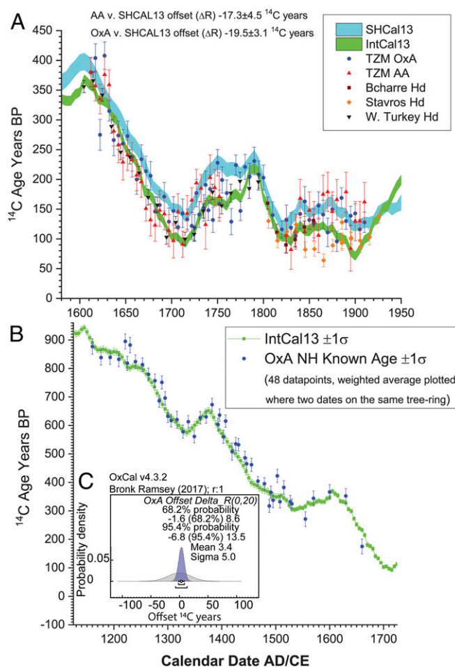
Fig. 3. (A) Comparison of the JJ ^{14}\text{C} data by laboratory versus both IntCal13 (1) and SHCal13 (2) ( 1\sigma errors shown). Known-age tree-ring ^{14}\text{C} measurements from Bcharré, (northern Lebanon), Stavros tis Psokas (western Cyprus), and Çatacık (western Turkey), are also shown (44). (B). OxA data on other known age NH tree rings (61, 62) versus IntCal13 (1). (C) Overall ^{14}\text{C} years offset OxA NH data in B versus IntCal13; light gray region shows the neutral prior ( 0 \pm 20 ) versus the calculated posterior region (blue) (27).
